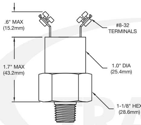
Dimensions In Inches And Are Reference Only.
