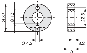
Fig 3-5: Spacer
