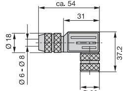
Fig. 3-2: Transducer BTL5...B/Z, Dimensions
