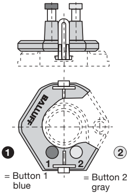
Fig. 6-1: Calibration device (shown on transducer)
