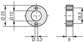
Fig. 3-4: Magnet (optional)
