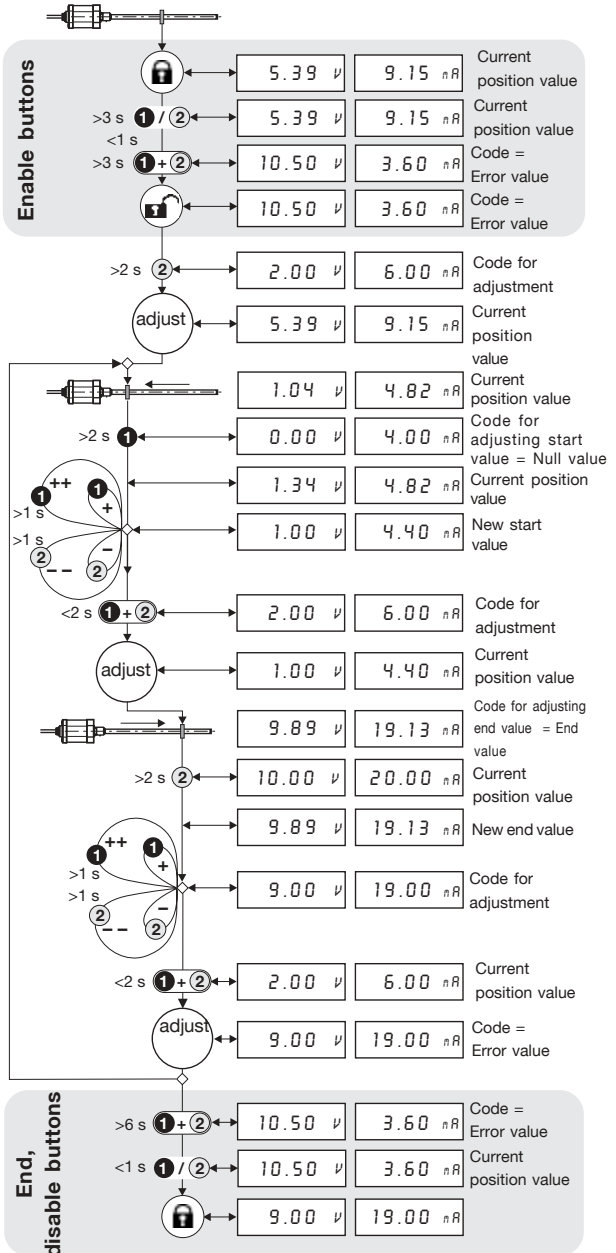
BTL5-A... with magnet in stroke range
