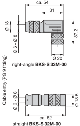
Fig. 4-3: Connector (optional)
