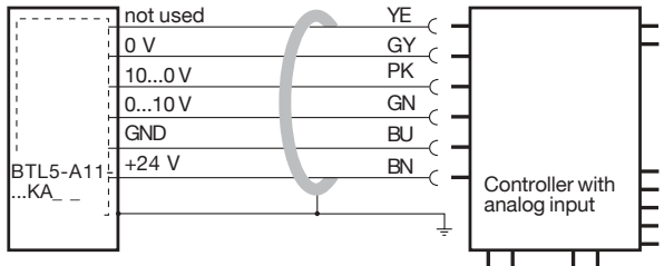
Fig. 4-1: BTL5-A11...KA__ with controller, wiring example
