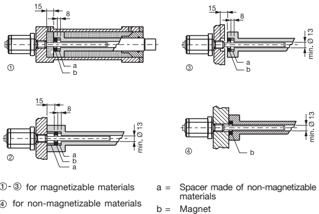
Fig. 3-1: Mounting
