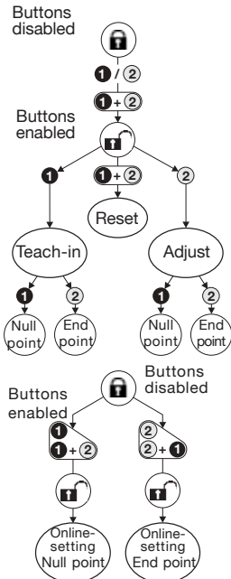
Fig. 6-3: Teach-in procedure
