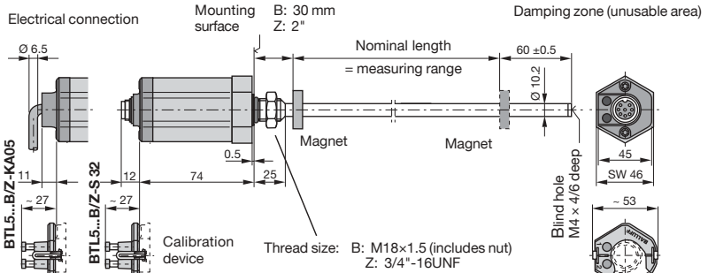
Fig. 3-2: Transducer BTL5...B/Z, Dimensions
