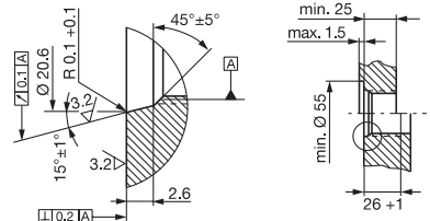
Fig. 3-3: Threaded hole for mounting the BTL with O-ring
