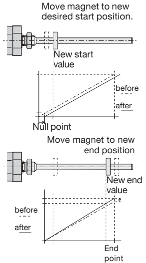
Fig. 6-4: Manual adjust procedure
